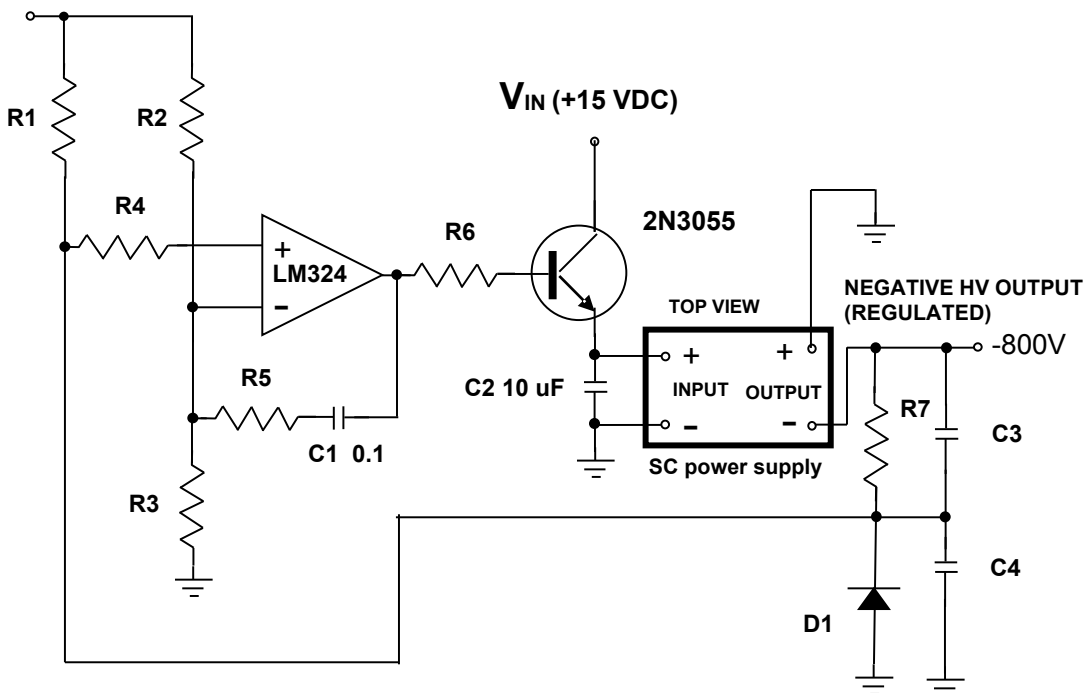
Figure 3: Negative 800 Volt Regulator
