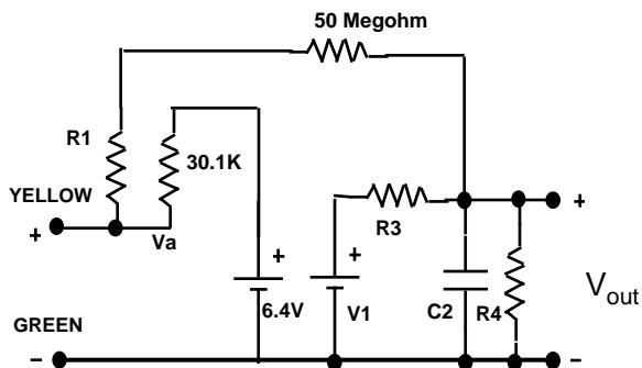
HTC Circuit Model
