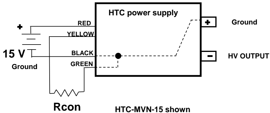
Figure 3: Resistance program of negative output of HTC
