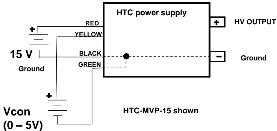
Figure 5: Voltage programming of positive output HTC
