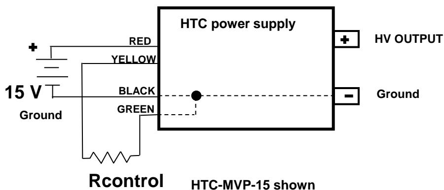
Figure 1: Resistance program of positive output of HTC
